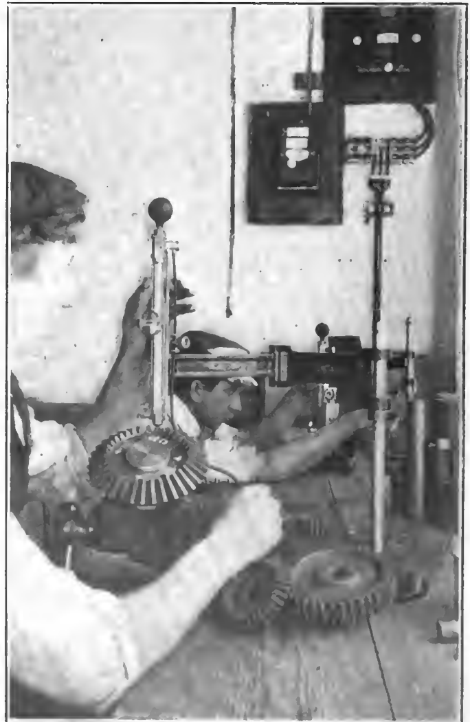
Fig. 2—Testing automobile gear teeth for hardness
